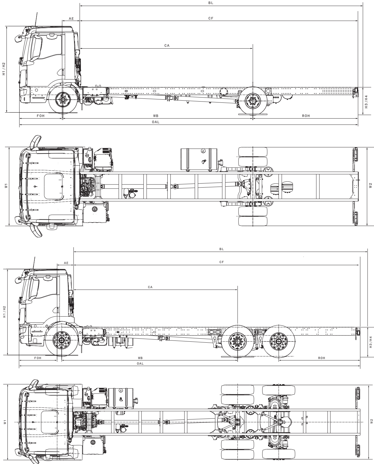
Illustration shows TGL 12.xxx 5200 4x2 CH NN vs TGM 26.xxx 5775 6x2-4 CH NN
